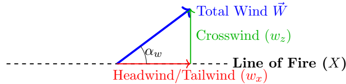
Figure 6.1: Decomposition of the total wind vector into range ( w_x ) and lateral ( w_z ) components. Only the w_z component causes side-to-side deflection.
