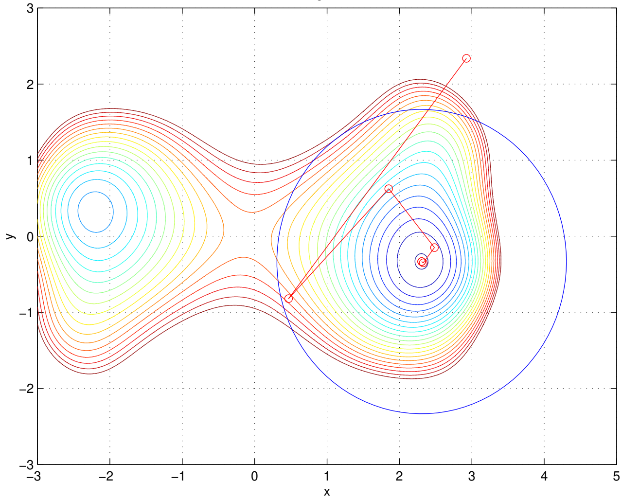
Trust-region method
