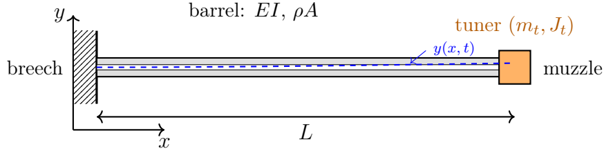
Figure 2: Barrel model: Euler-Bernoulli beam clamped at the breech ( x = 0 ), free at the muzzle ( x = L ), carrying at its end a point mass and its rotational inertia ( m_t, J_t ) representing the tuner. The dashed curve illustrates a transverse deflection y(x, t) .
