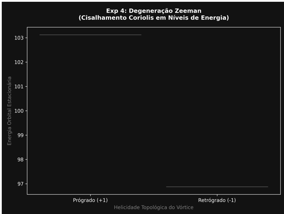
Figure 5: Mechanical bifurcation of formerly degenerate energy levels into distinct split frequencies via purely directional fluid friction.
