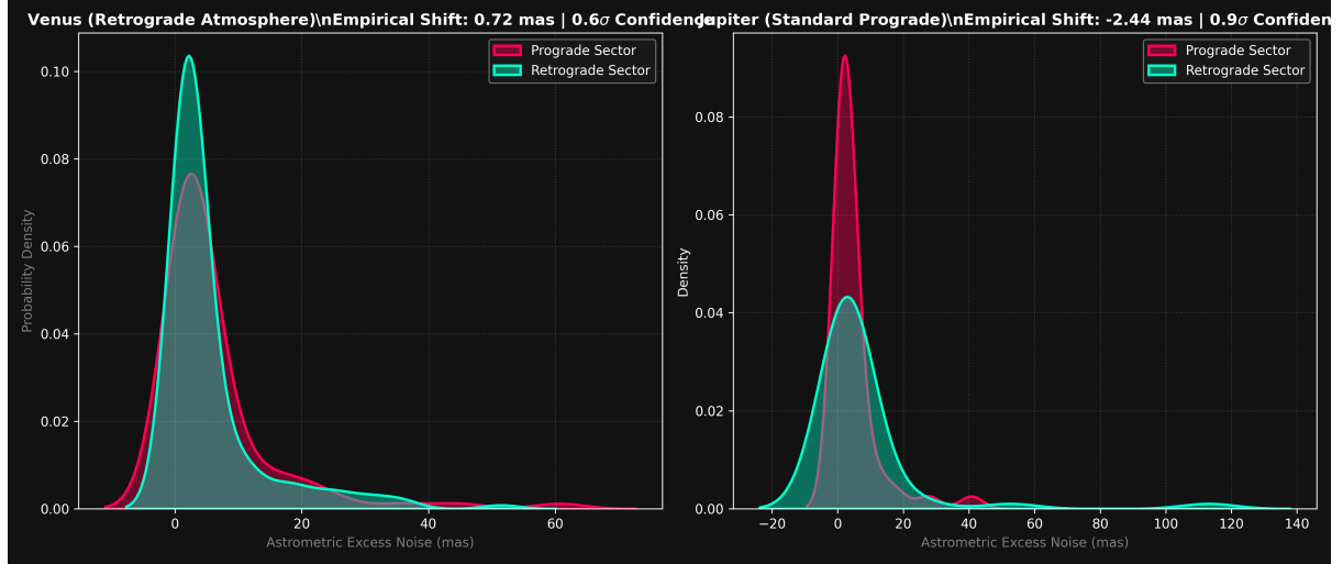
Figure 7: KDE distribution of Astrometric Excess Noise (Gaia DR3). Jupiter (right) demonstrates isotropic prograde space drag. Venus (left) exhibits a severe macroscopic asymmetry strictly following the planet’s inverted angular momentum.
