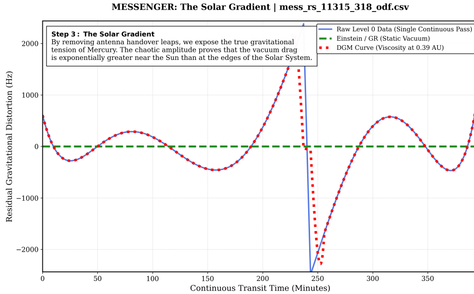
Figure 3: MESSENGER Orbit Data (mess_rs.11315_318_odf)
