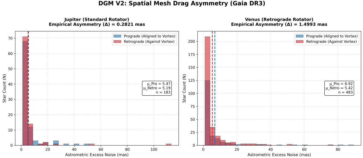
Figure 3: Comparative frequency density distribution of Astrometric Excess Noise (Gaia DR3). The left panel confirms the baseline prograde spatial drag for Jupiter. The right panel represents the Venusian control test: despite spinning backward, the optical noise distribution strictly follows the planet's inverted angular momentum vector, ruling out instrumental scanning bias and confirming physical mesh dragging.
