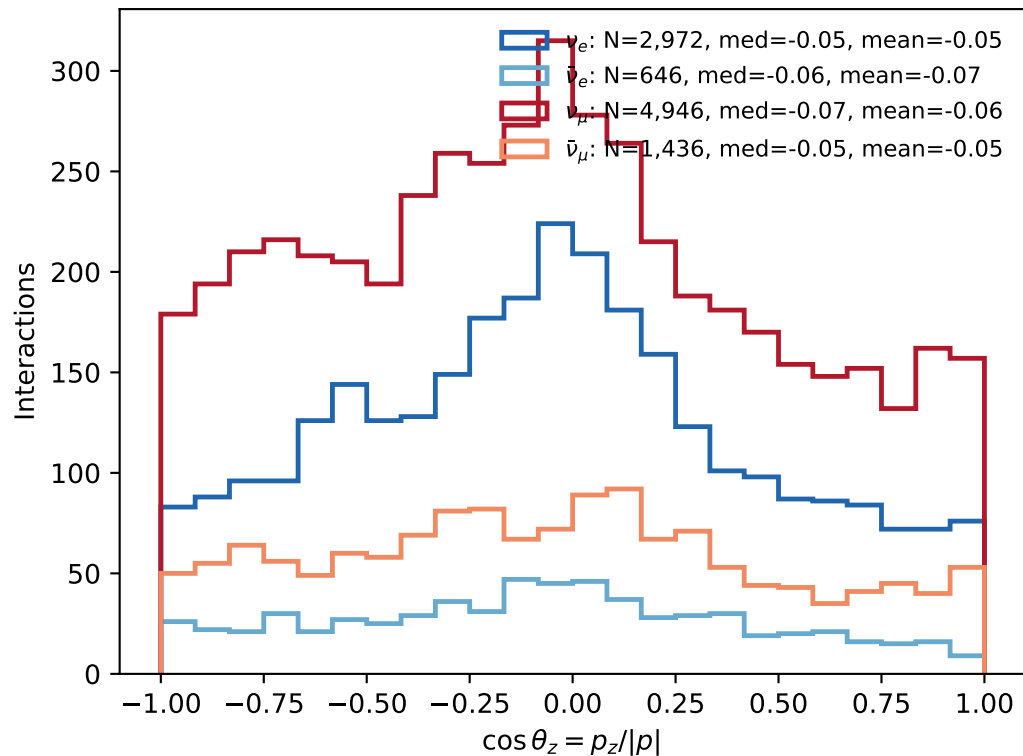
Incoming detector-coordinate direction
