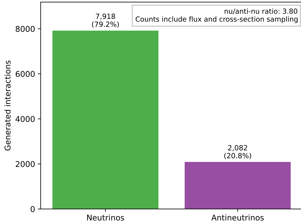
Neutrino versus antineutrino
