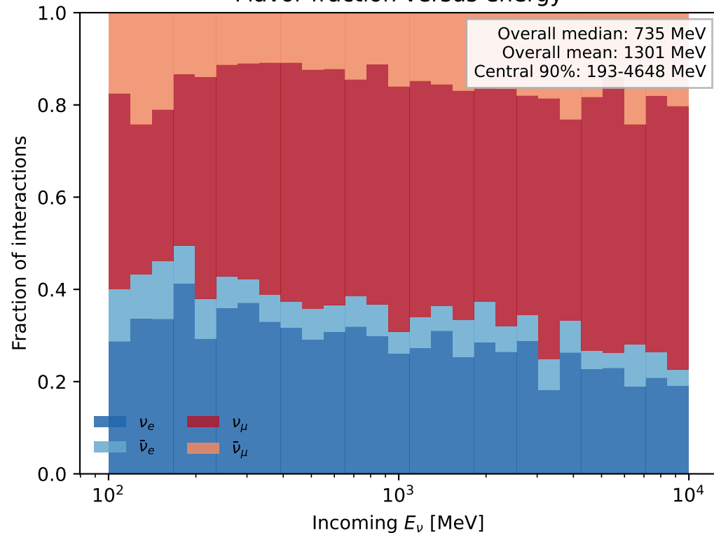
Flavor fraction versus energy
