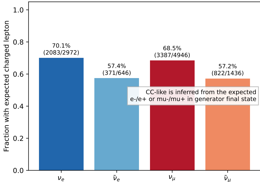
Charged-current-like outcome
