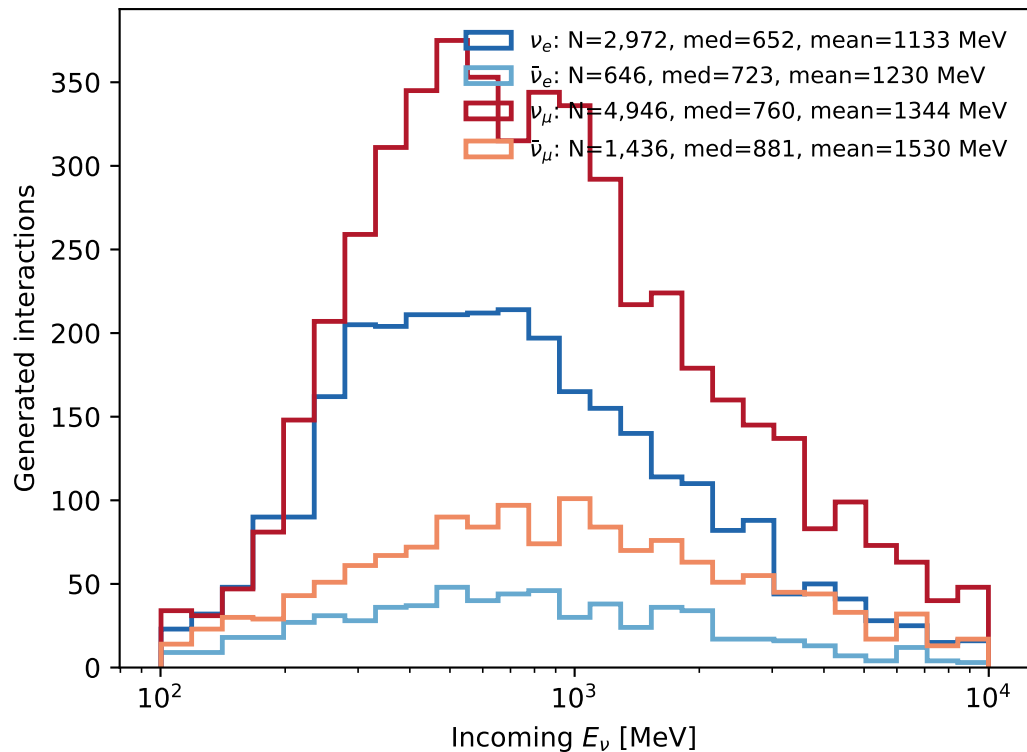
Incoming energy by flavor
