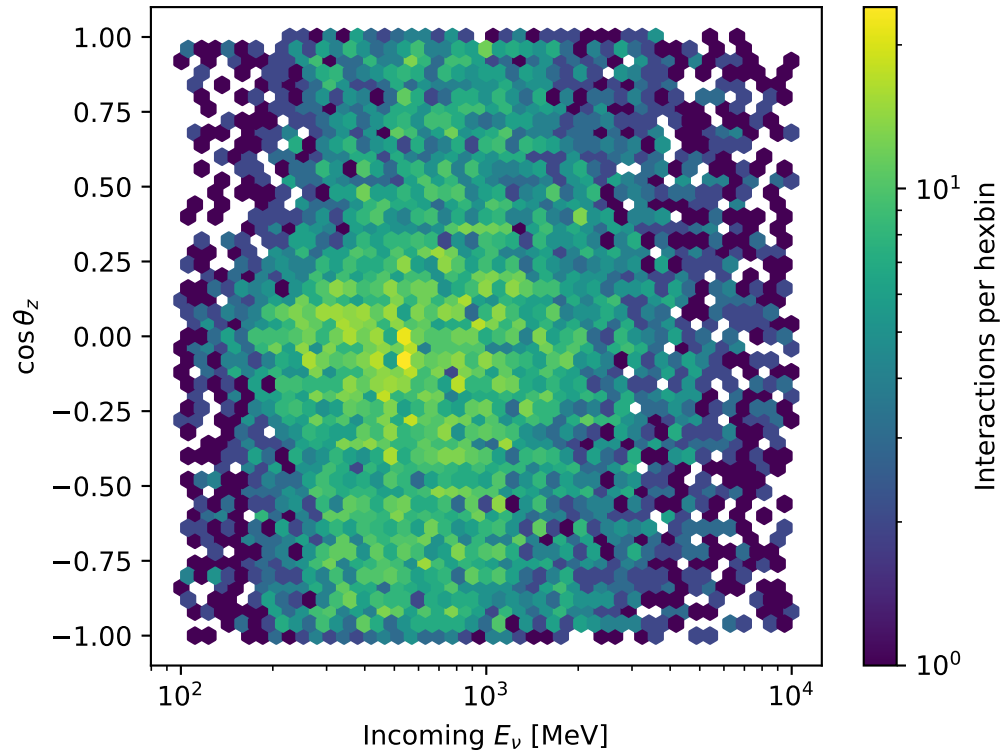
Energy versus direction
