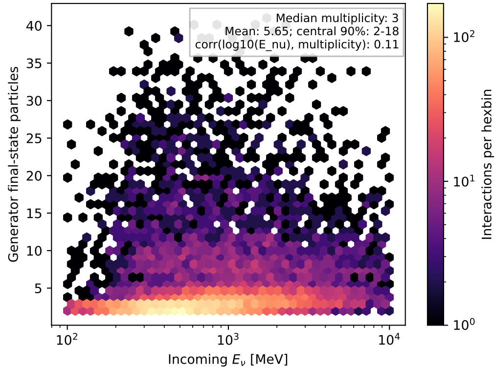
Final-state multiplicity versus energy
