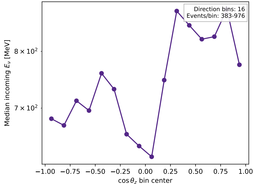
Median energy versus direction
