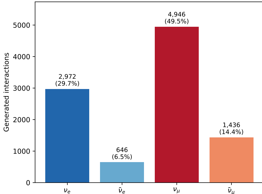
Incoming flavor composition
