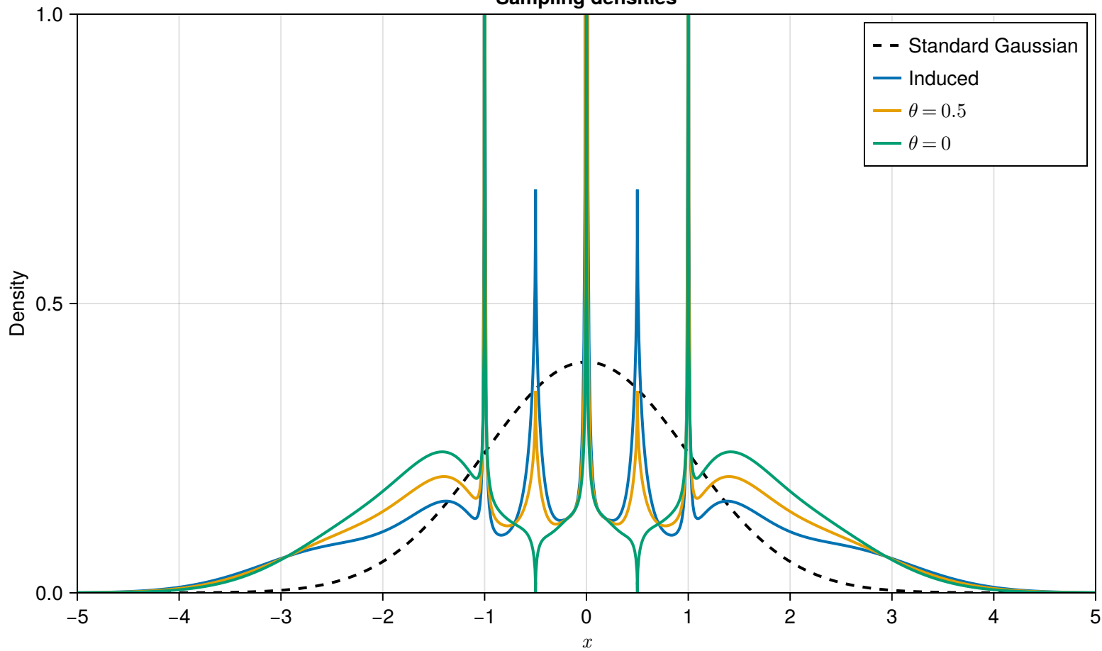
Sampling densities
