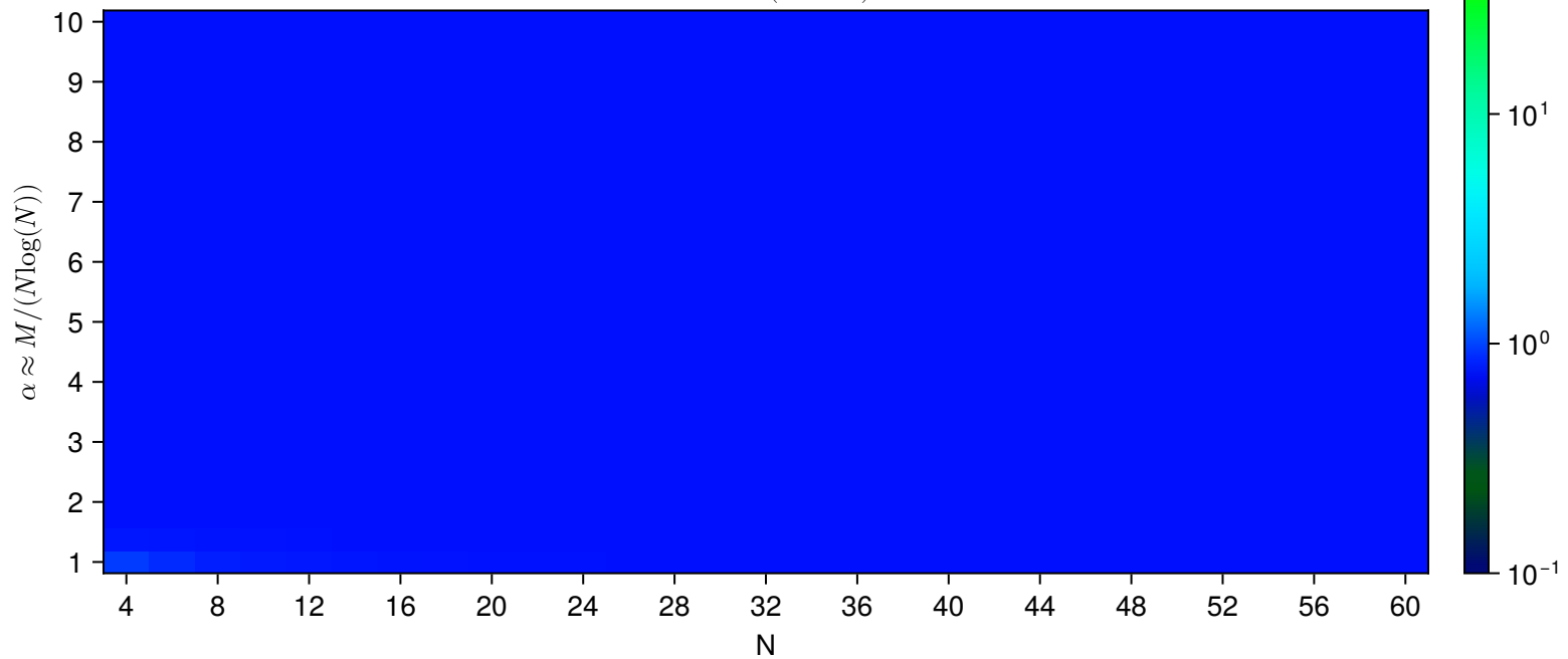
Mixture ( \theta = 0.5 )
