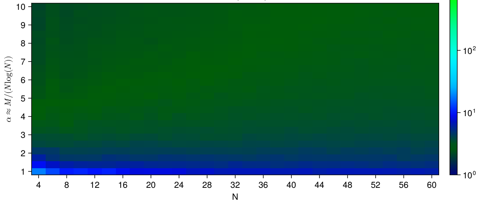
Mixture ( \theta = 0.5 )
