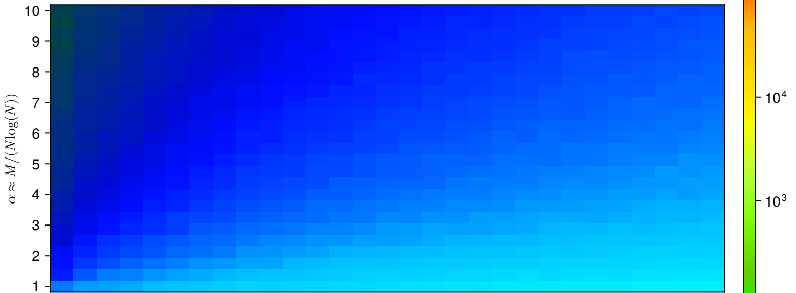
Mixture ( \theta = 0.5 )
