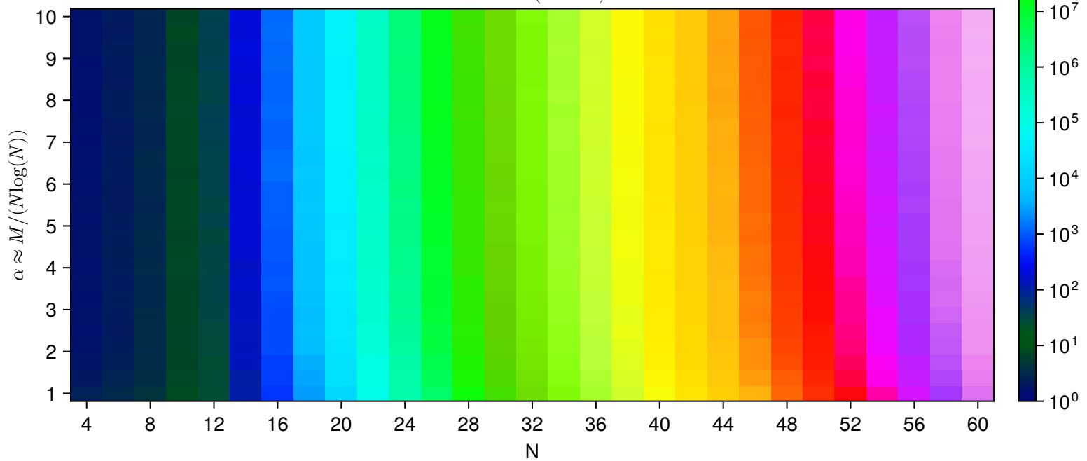
Mixture ( \theta = 0.5 )
