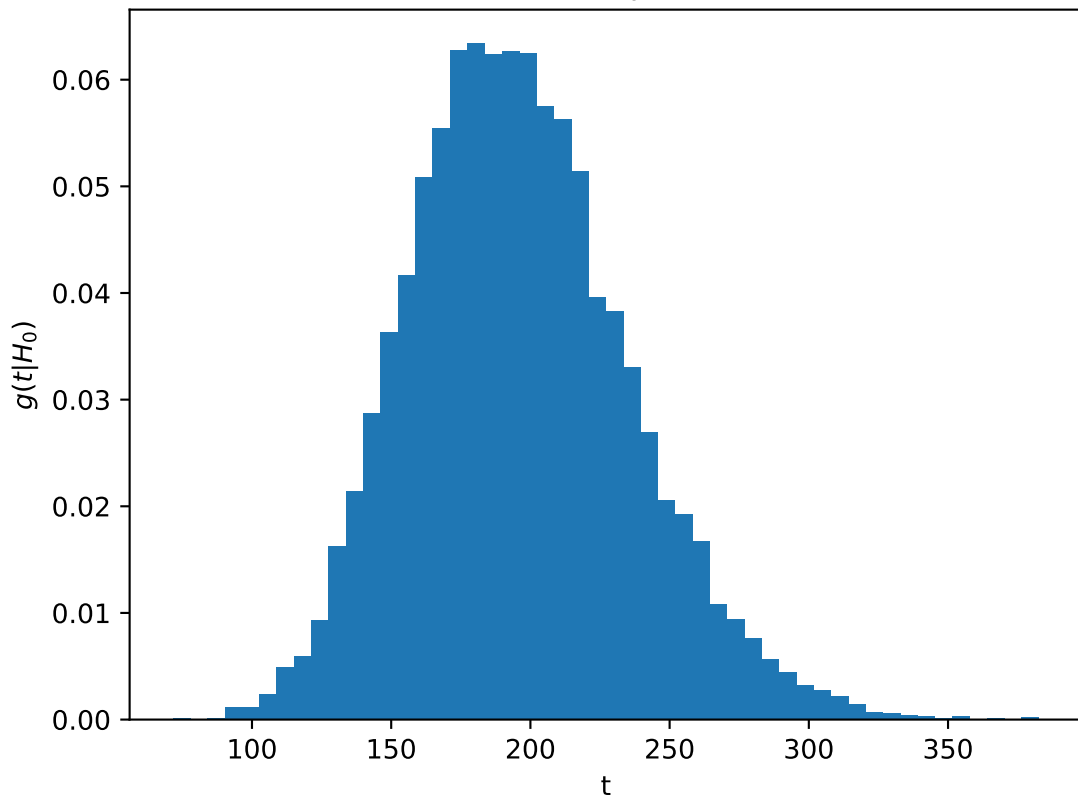
10000 MC experiments
