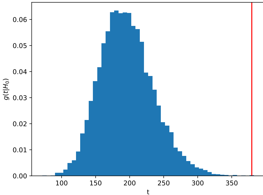
Critical region for 5\sigma significance
