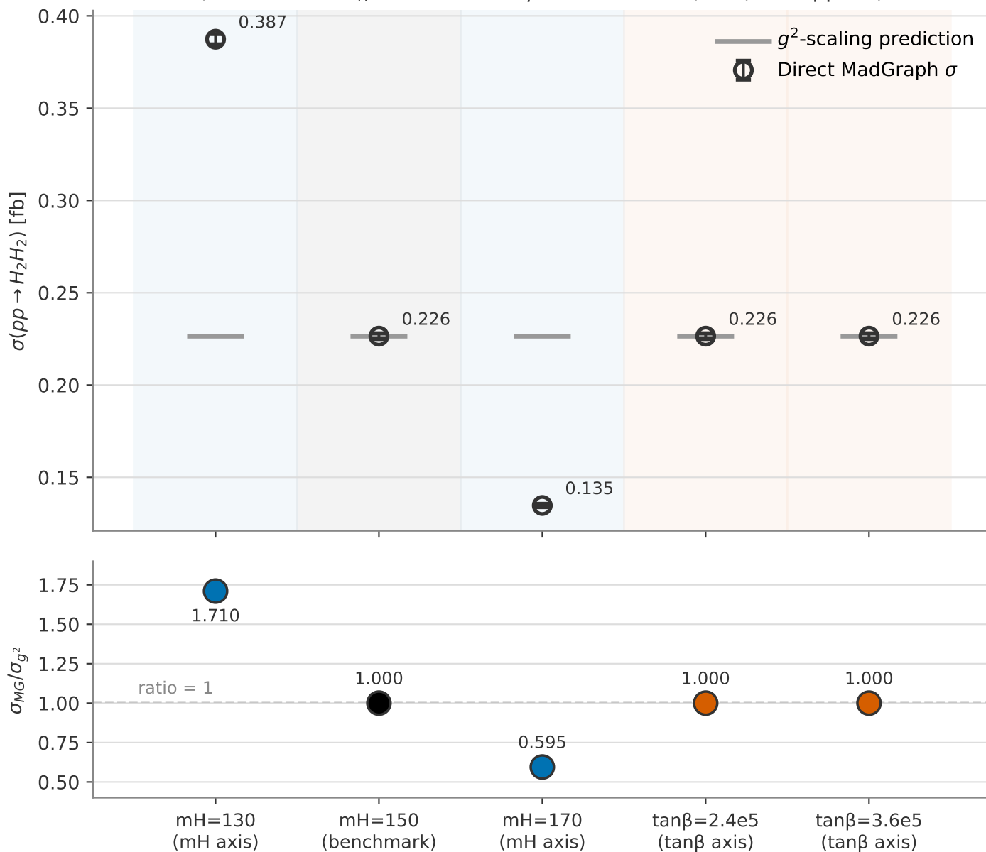
Direct MadGraph \sigma vs. g^2 -scaling prediction (benchmark: m_H=150 GeV, \tan\beta=3\times 10^5 ; A \times \varepsilon(\text{ctau}) not applied)
