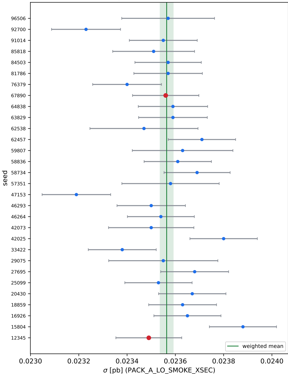
Pack A seed ensemble: per-seed cross section \pm reported MG5 error
