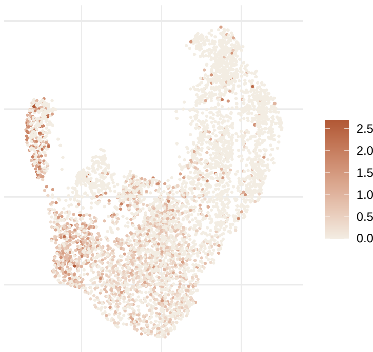
BATF
