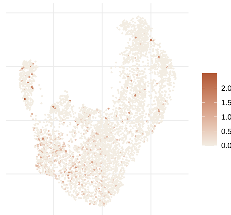
ATF3
