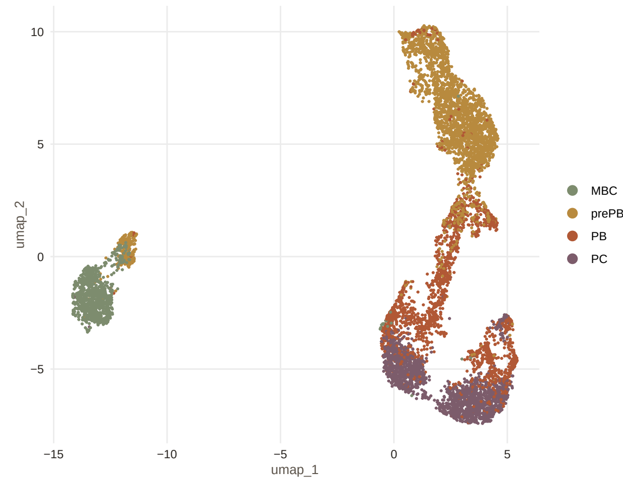
Headline UMAP: by stage
