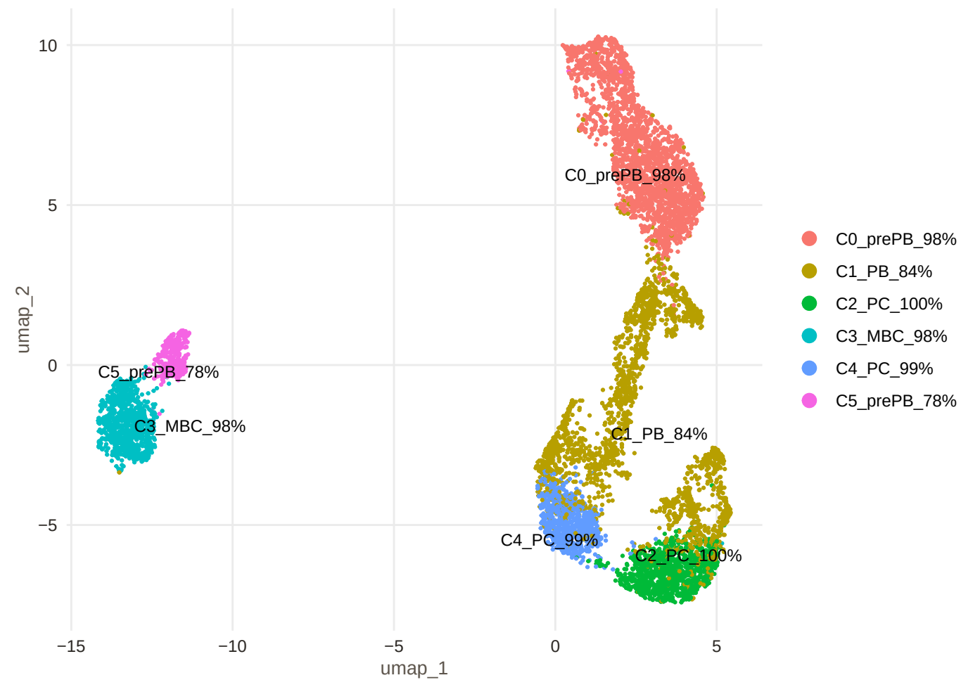
Headline UMAP: annotated clusters
