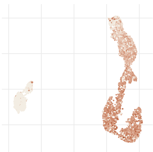
MZB1
