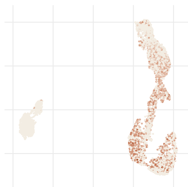
TNFRSF17
