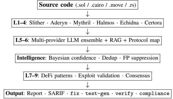
Fig. 1. MIESC pipeline: 9 defense layers with multi-provider LLM ensemble and intelligence engine for cross-tool confidence scoring.
