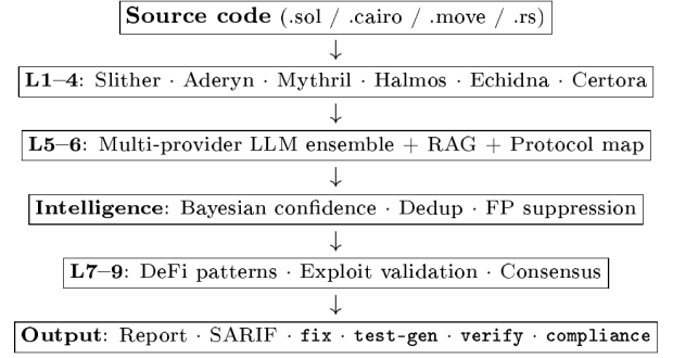
Fig. 1. MIESC pipeline: 9 defense layers with multi-provider LLM ensemble and intelligence engine for cross-tool confidence scoring.
