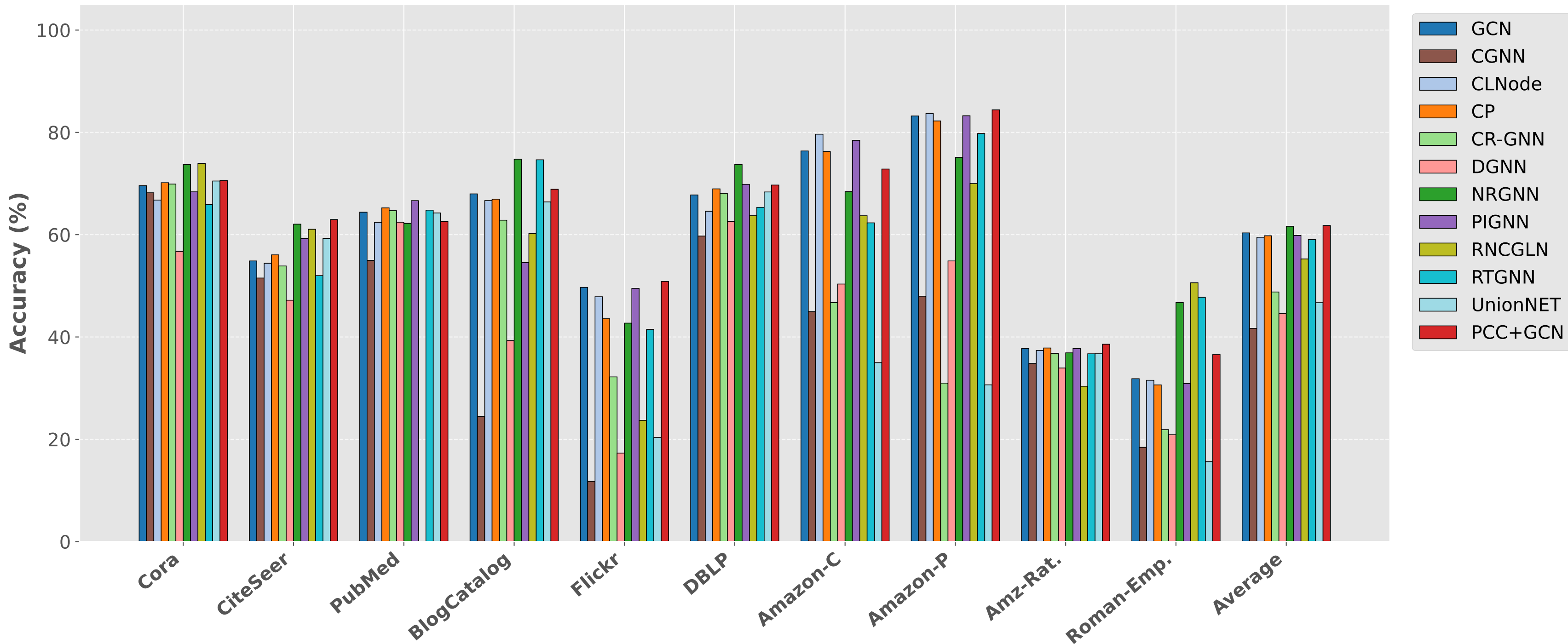
Mean Accuracy Comparison: UNIFORM Noise
