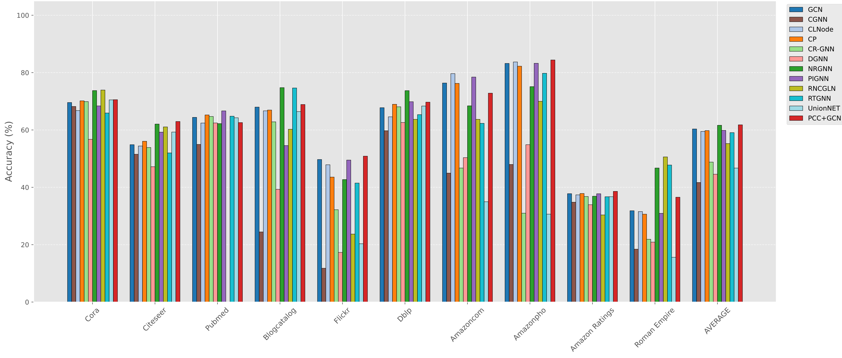
Mean Accuracy Comparison: UNIFORM Noise
