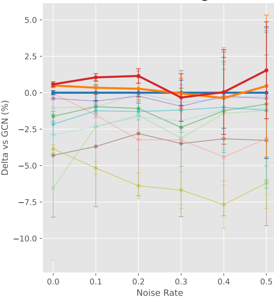
Amazon Ratings
