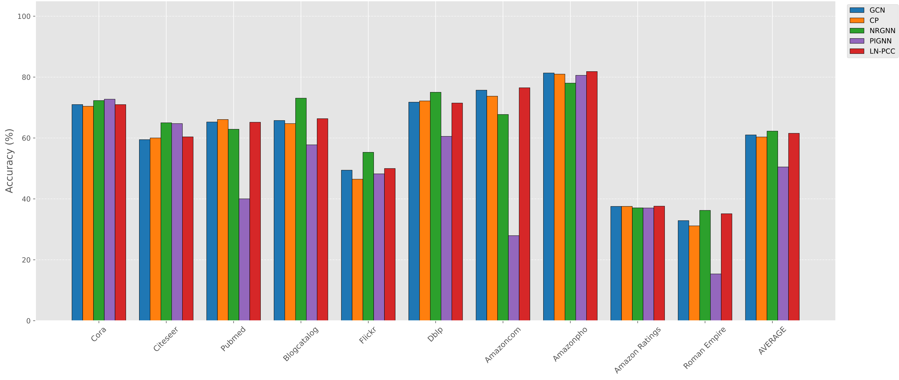
Mean Accuracy Comparison: INSTANCE Noise
