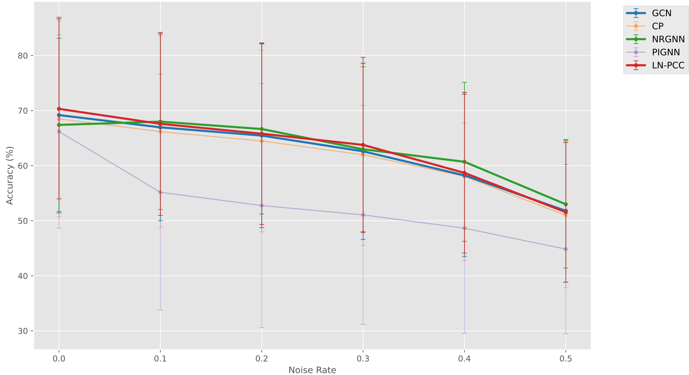
Instance Noise Global Summary (Accuracy)
