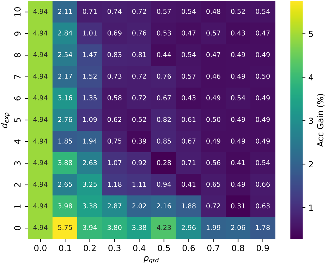
Noise 30%
