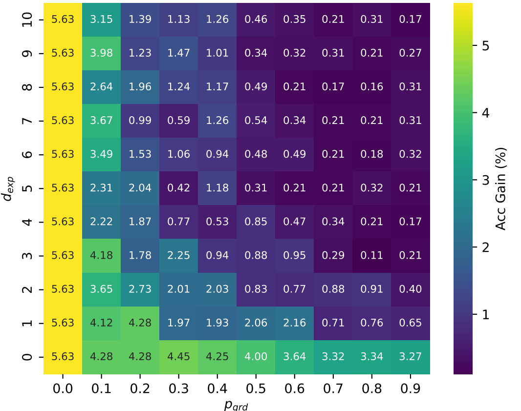
Noise 40%
