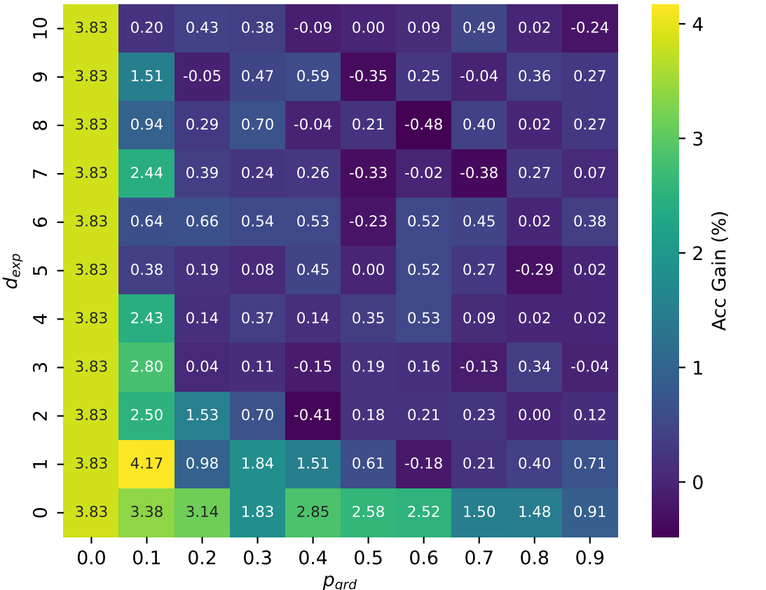
Noise 50%
