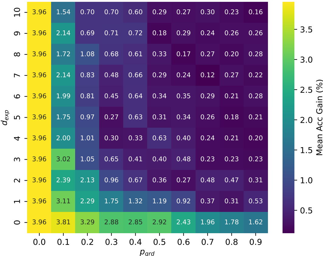
GLOBAL MEAN
