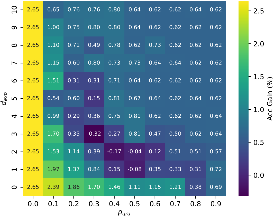
Noise 10%
