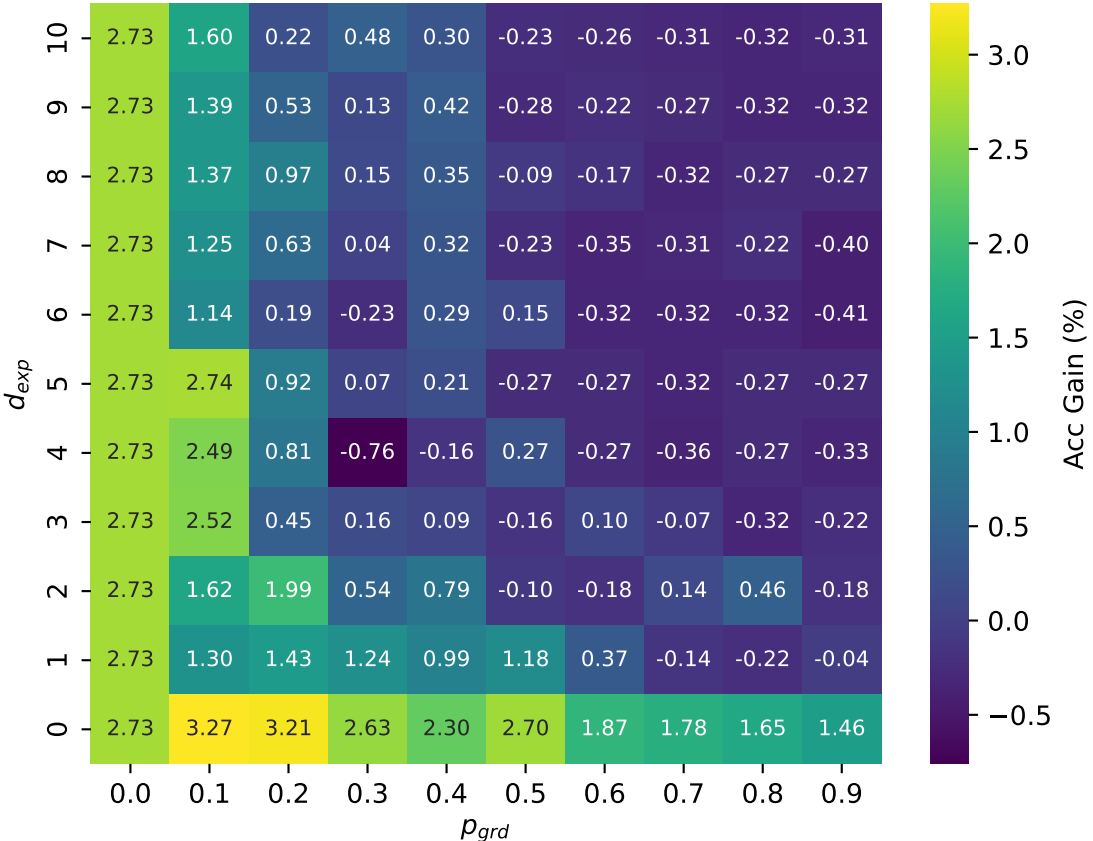
Noise 20%
