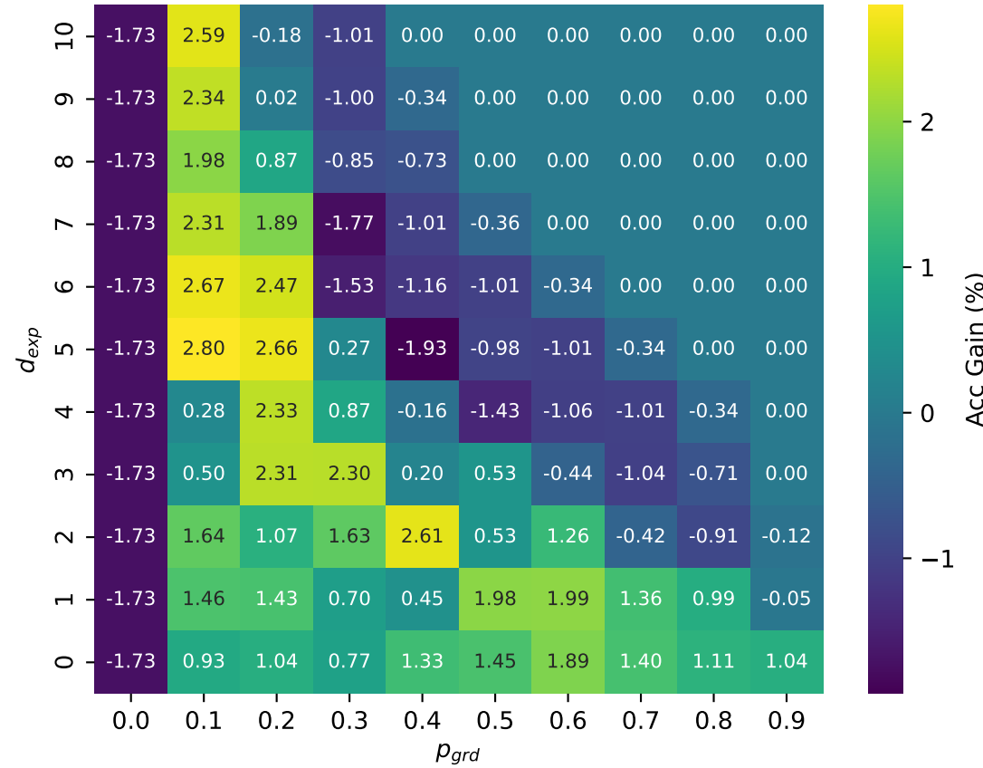
Noise 50%
