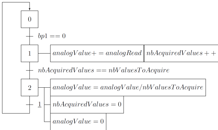
Figure: Prog. 4 - Acquisition grandeurs analogiques
