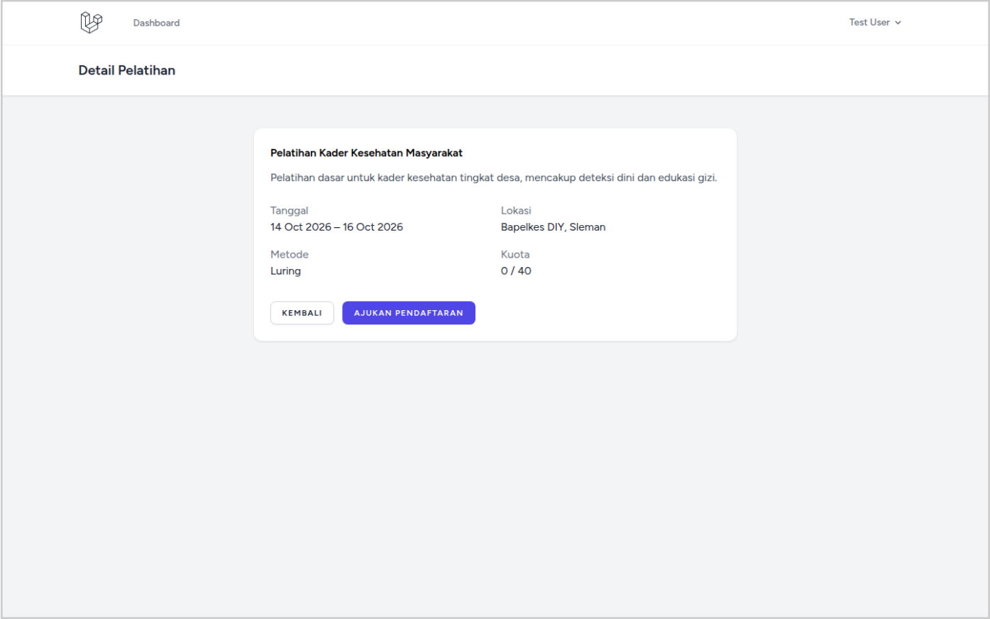
Desktop (1440x900)
