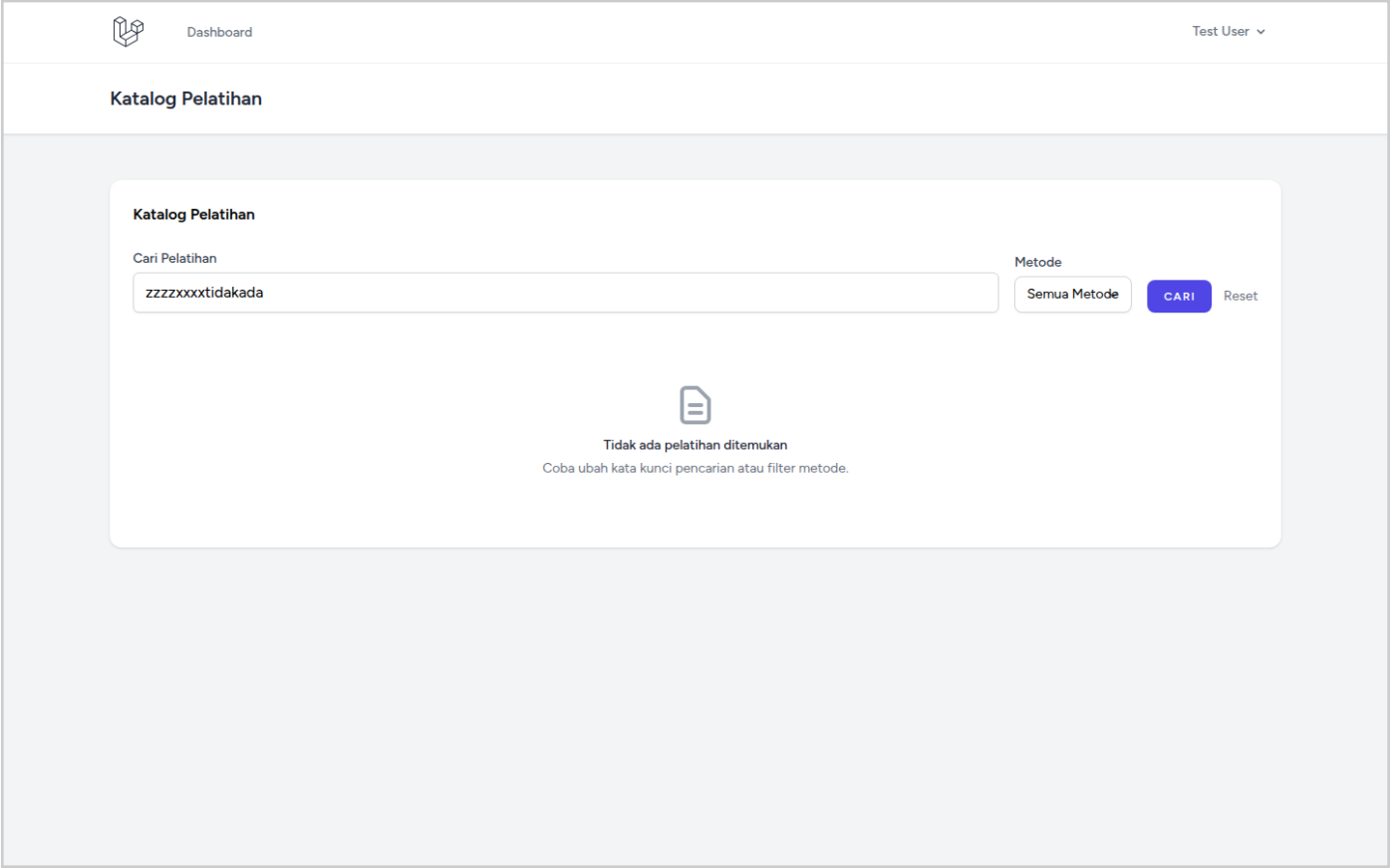
Desktop (1440×900)
