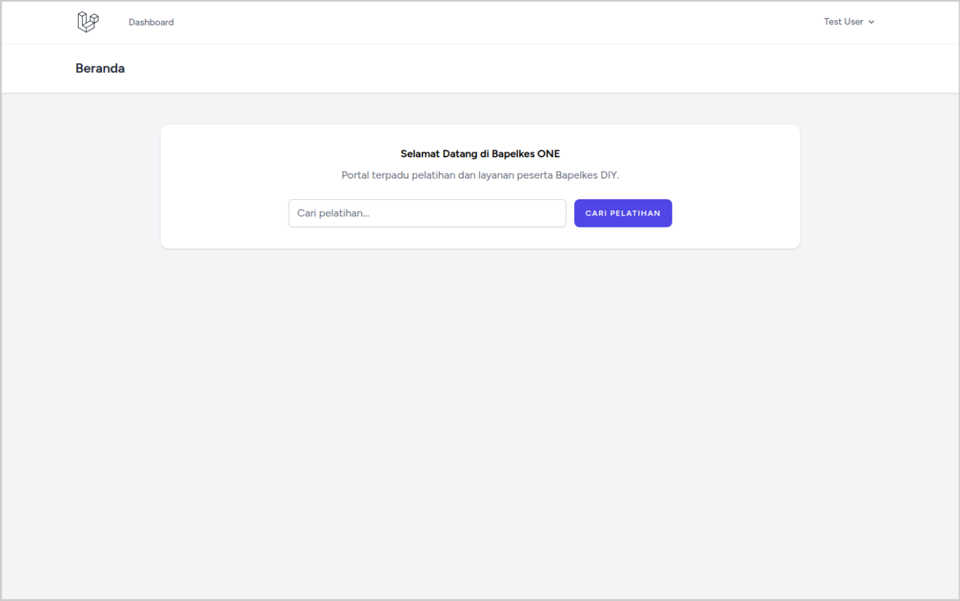
Desktop (1440×900)
