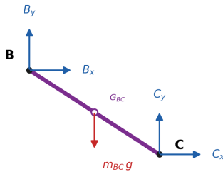
(c) Balancín BC
