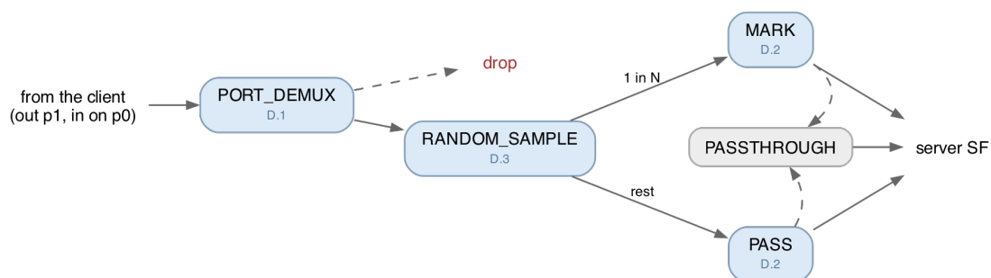
Figure 3: The Part D pipeline. Solid arrows are where a packet goes when it matches, dashed ones where it goes when it does not.
