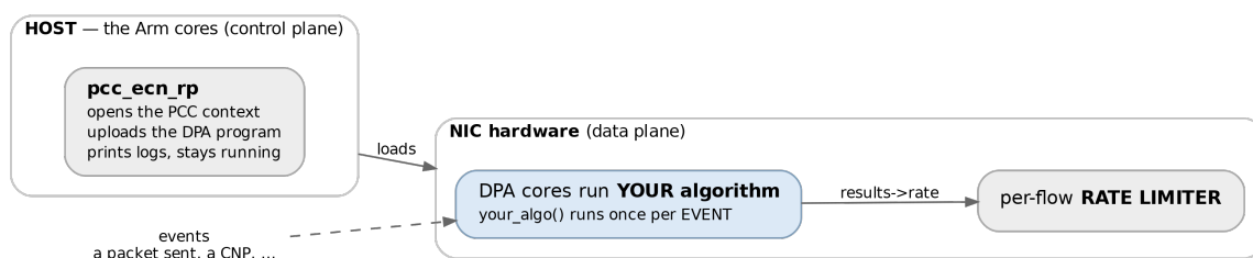
Figure 1: The two halves of a DOCA PCC program. The host side only loads and supervises; every packet-time decision happens on the DPA, inside the algorithm you write.
