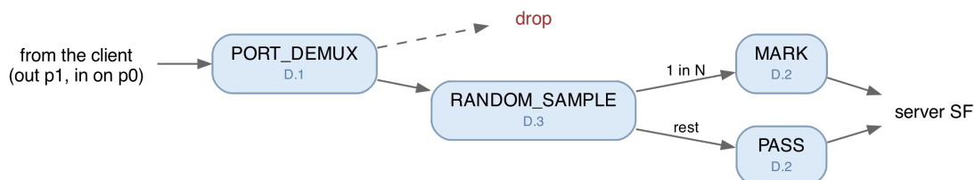
Figure 3: The Part D pipeline. Solid arrows are where a packet goes when it matches, dashed ones where it goes when it does not.
