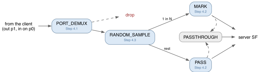
Figure 3: The Step 4 pipeline. Solid arrows are where a packet goes when it matches, dashed ones where it goes when it does not.
