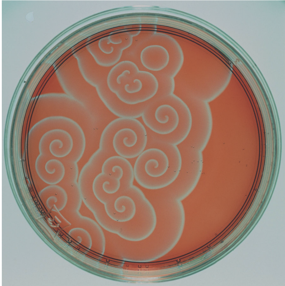
Figure 1: Belousov-Zhabotinsky reaction pattern
