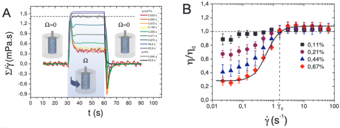
(a) Shear stress \Sigma rescaled by the applied shear rate \dot{\gamma} during the rotation to display an effective viscosity \Sigma/\dot{\gamma} in the sheared regime. (b) Relative viscosity \eta/\eta_0 averaged over three realisations as a function of \dot{\gamma} .
