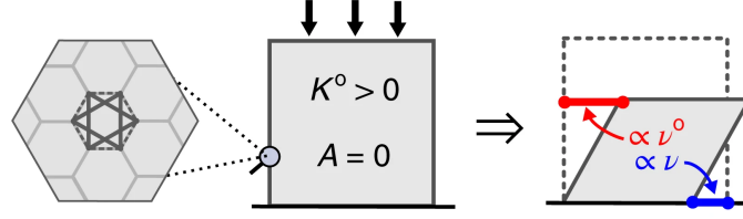
Figure 3: Demonstration of odd elasticity in active materials. When a vertical force is applied (downward arrow), the material not only compresses vertically but also generates a perpendicular displacement (horizontal arrow). This coupling between orthogonal deformations, characterized by the antisymmetric component of the elastic modulus tensor C_{ij}^{\text{odd}} , is impossible in passive materials where energy conservation requires symmetric response. In active materials, continuous energy injection breaks time-reversal symmetry, enabling this exotic mechanical behavior where stress in one direction induces strain in perpendicular directions.
