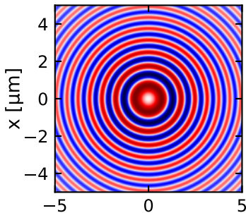
Spherical wave
