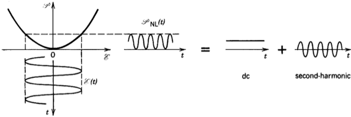
Figure 2: Second-order polarization effects. The input electric field E(t) (left) creates a nonlinear polarization \hat{P}^{(2)}(t) (right) with two components: one oscillating at twice the input frequency (second harmonic generation) and a static component (optical rectification).
