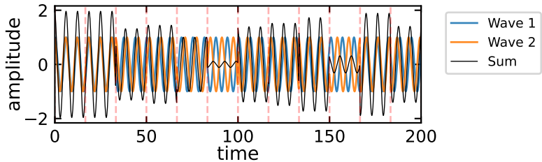
Superposition with Multiple Phase Jumps
