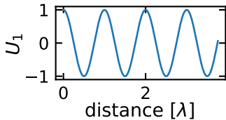
Destructive ( \Delta\phi = \pi )
