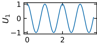
Constructive ( \Delta\phi = 0 )
