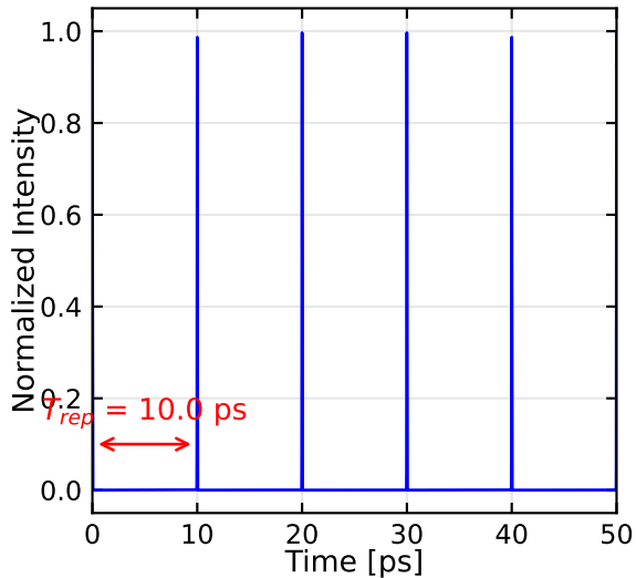
Pulse Train (Time Domain)
