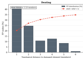
Topological Distance Distribution of False Positive Nodes
