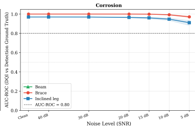
DQI Robustness: AUC-ROC Degradation vs. Noise Level (SNR)
