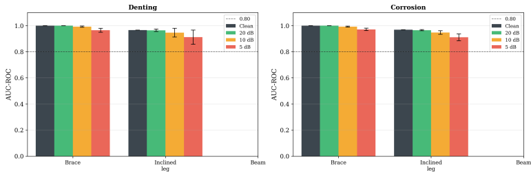
AUC-ROC Comparison: Clean vs Noisy DQI (20 dB and 10 dB SNR)
