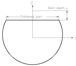
Figure 1: Parametrisation of the dented cross-section.
