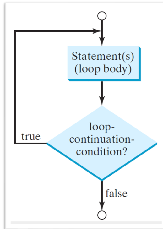
do-while Loop
