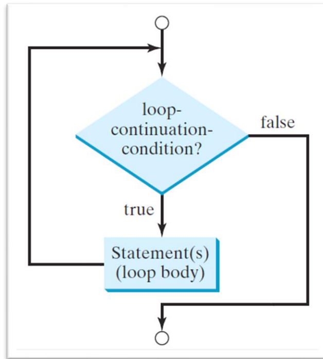
while Loop
