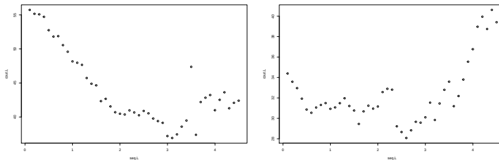
Figure: Maintenance cost in function of the preventive threshold L , with \tau = 0.5 (left) and \tau = 0.8 (right): M = 5 , \alpha = 1 , \beta = 1 , b = 1 .
