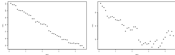
Figure: Maintenance cost in function of the preventive threshold L , with C_p = \frac{C_c}{2} (left) and C_p = \frac{C_c}{5} (right) and \tau = 0.8 : M = 5 , \rho = 0.8 , \alpha = 1 , \beta = 1 , b = 1 .
