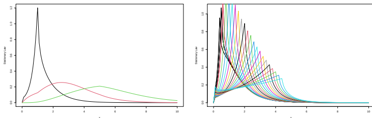
Figure: The steady-state distribution in function of the inspection interval \tau (left) and the preventive threshold L (right): M = 5 , \rho = 0.8 , \alpha = 1 , \beta = 1 , b = 1 .
