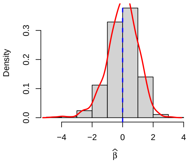
Case 1 (transformed data): \alpha = 1.0 , \beta = 1.0 , b = 1.0 , \rho = 0.2
