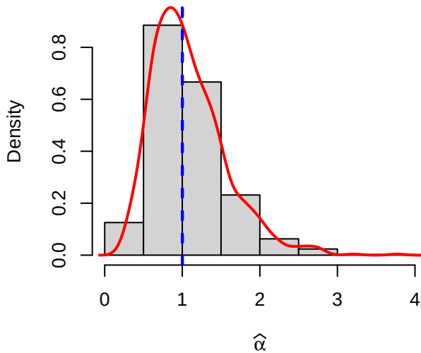
Case 4: \alpha = 1.0 , \beta = 0.75 , b = 1.0 , \rho = 0.2
