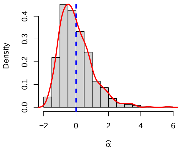
Case 4 (transformed data): \alpha = 1.0 , \beta = 0.75 , b = 1.0 , \rho = 0.2
