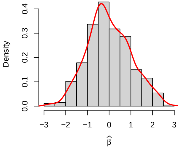
Case 6 (transformed and normalized data): \alpha = 1.0 , \beta = 0.75 , b = 1.0 , \rho = 0.8
