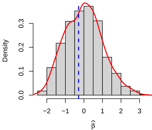
Case 5 (transformed data): \alpha = 1.0 , \beta = 0.75 , b = 1.0 , \rho = 0.5
