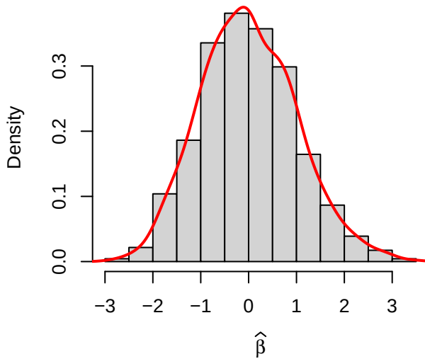
Case 4 (transformed and normalized data): \alpha = 1.0 , \beta = 0.75 , b = 1.0 , \rho = 0.2
