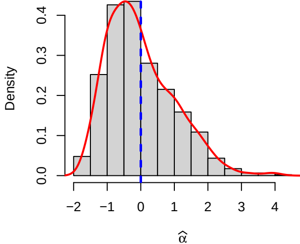
Case 5 (transformed data): \alpha = 1.0 , \beta = 0.75 , b = 1.0 , \rho = 0.5
