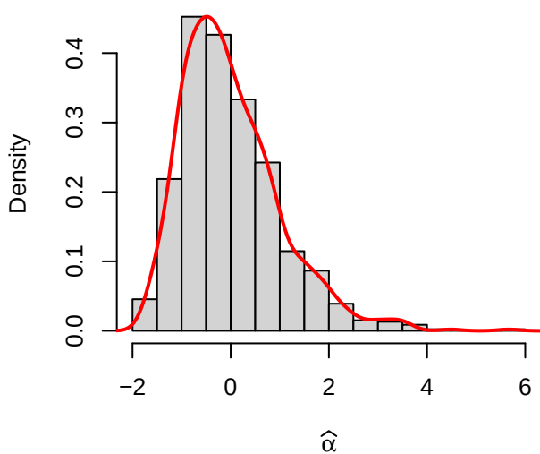
Case 4 (transformed and normalized data): \alpha = 1.0 , \beta = 0.75 , b = 1.0 , \rho = 0.2
