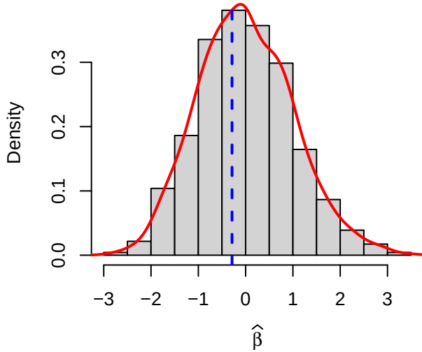
Case 4 (transformed data): \alpha = 1.0 , \beta = 0.75 , b = 1.0 , \rho = 0.2
