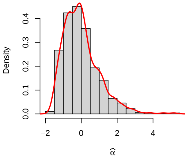
Case 6 (transformed and normalized data): \alpha = 1.0 , \beta = 0.75 , b = 1.0 , \rho = 0.8
