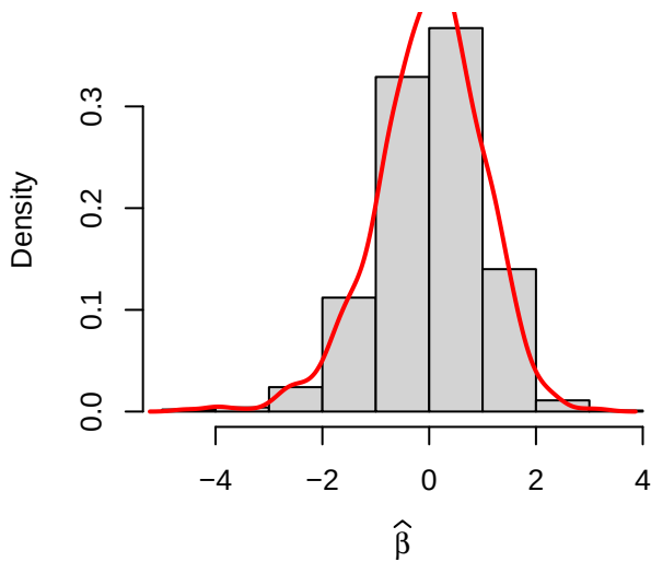
Case 1 (transformed and normalized data): \alpha = 1.0 , \beta = 1.0 , b = 1.0 , \rho = 0.2
