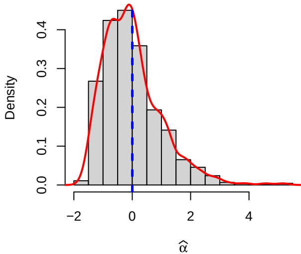
Case 6 (transformed data): \alpha = 1.0 , \beta = 0.75 , b = 1.0 , \rho = 0.8
