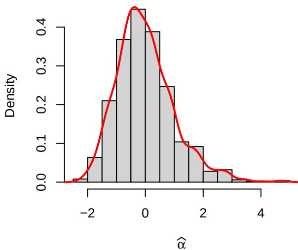
Case 9 (transformed and normalized data): \alpha= 1.0 , \beta= 1.2 , b= 1.0 , \rho= 0.8
