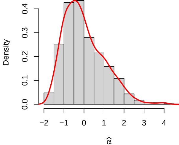
Case 5 (transformed and normalized data): \alpha = 1.0 , \beta = 0.75 , b = 1.0 , \rho = 0.5
