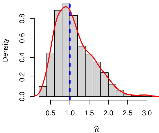
Case 5: \alpha= 1.0 , \beta= 0.75 , b= 1.0 , \rho= 0.5
