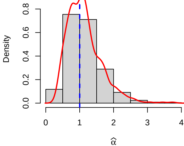
Case 6: \alpha=1.0 , \beta=0.75 , b=1.0 , \rho=0.8
