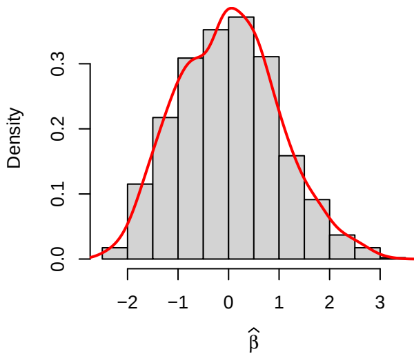
Case 5 (transformed and normalized data): \alpha = 1.0 , \beta = 0.75 , b = 1.0 , \rho = 0.5
