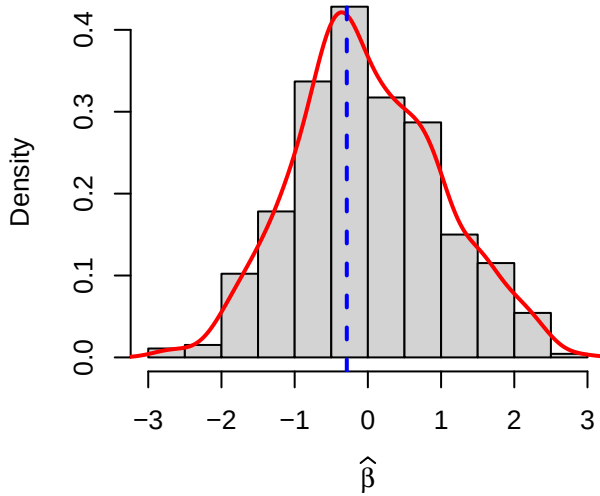
Case 6 (transformed data): \alpha = 1.0 , \beta = 0.75 , b = 1.0 , \rho = 0.8
