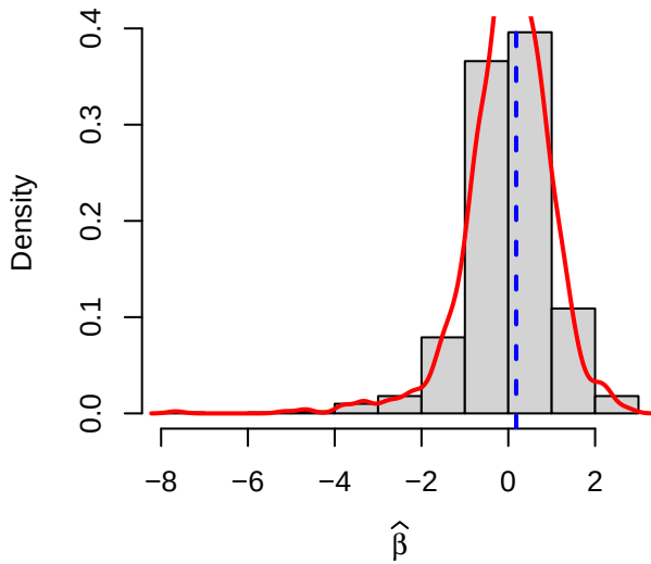
Case 7 (transformed data): \alpha= 1.0 , \beta= 1.2 , b= 1.0 , \rho= 0.2
