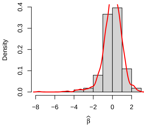
Case 7 (transformed and normalized data): \alpha = 1.0 , \beta = 1.2 , b = 1.0 , \rho = 0.2
