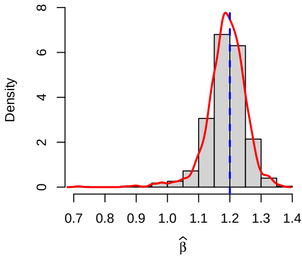
Case 7: \alpha = 1.0 , \beta = 1.2 , b = 1.0 , \rho = 0.2
